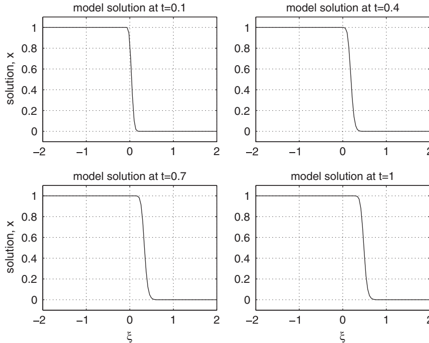
Figure 1. Burgers model solutions for Reynolds number Re=50 at different time steps.
