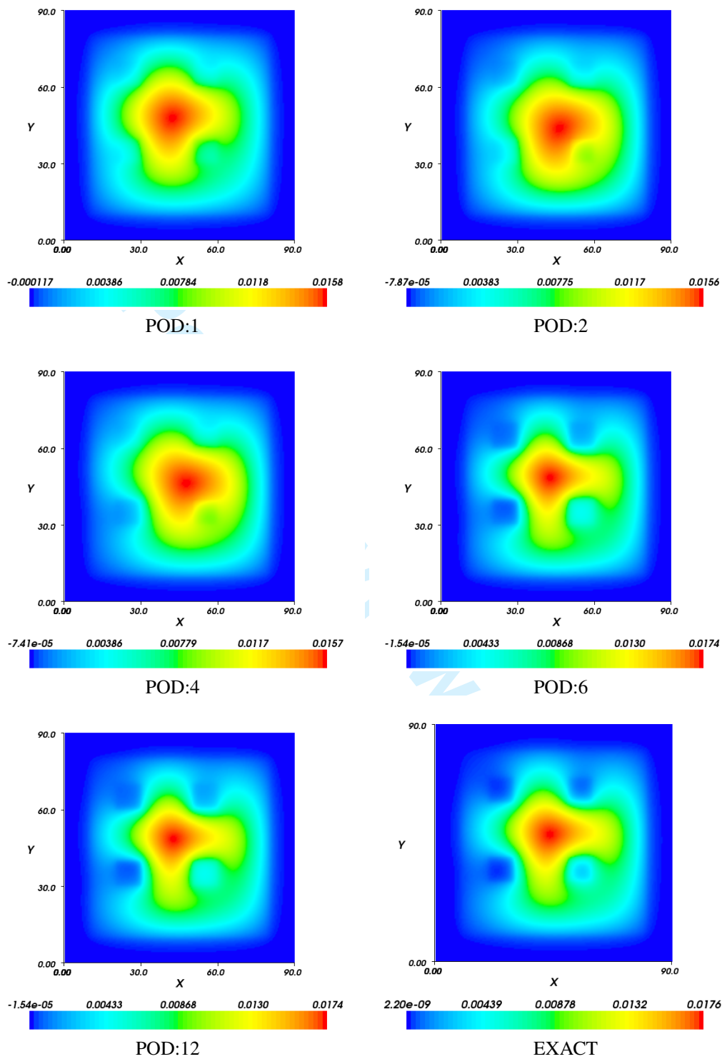
Figure 14. The reference solution of problem R7 together with its POD representation using varying expansion sizes.
