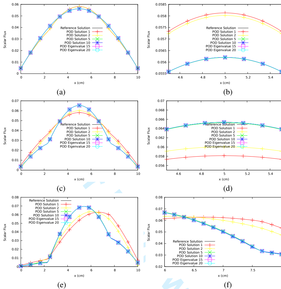
Figure 6. The reduced order solutions of the normalised scalar flux eigenfunction for problems R1 (a,b), R2 (c,d) and R3 (e,f). Both the full solutions are shown together with their localised views which aim to highlight the regions with the largest errors. The numbers in the legend indicates the number of POD functions used in the reduced order model.
