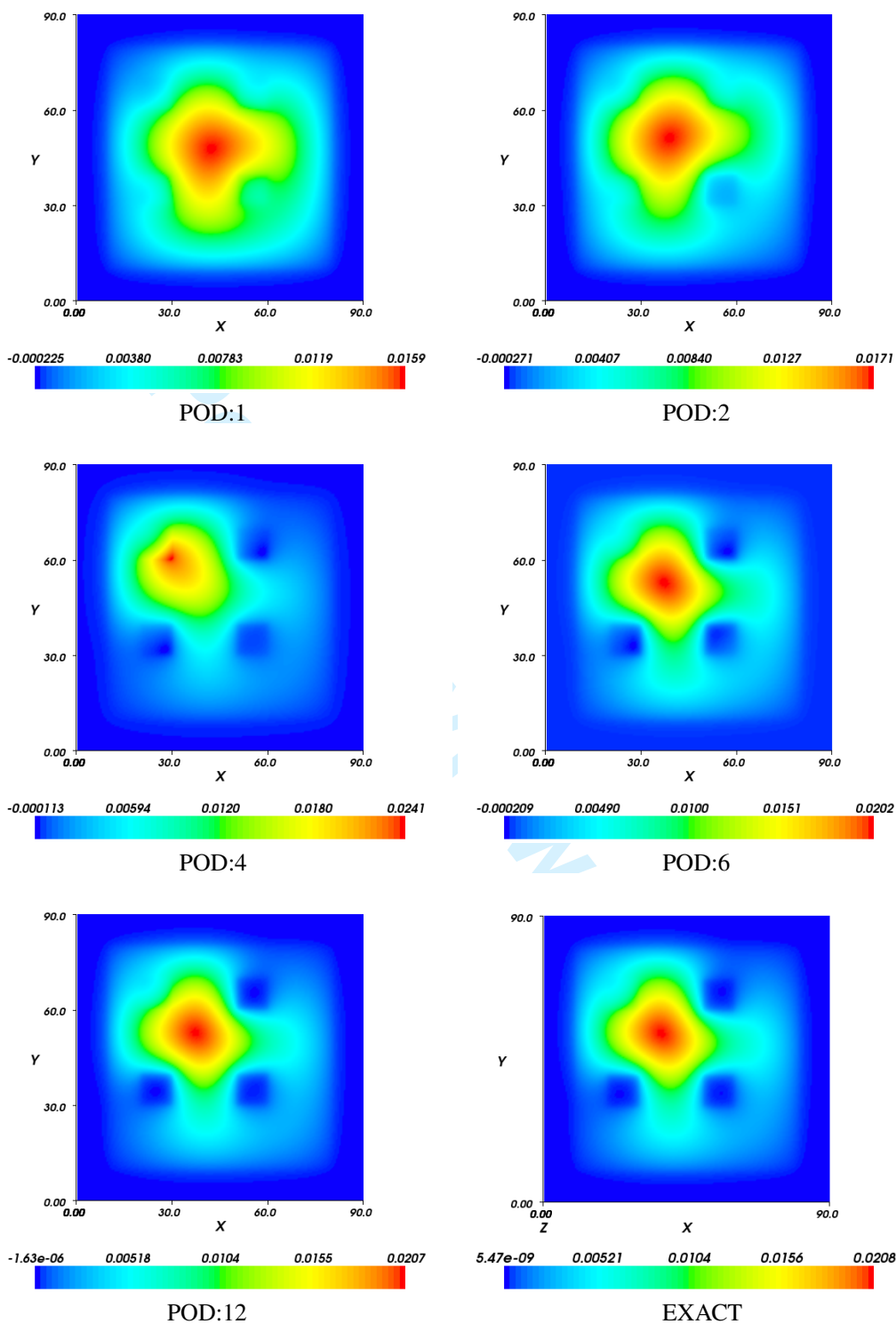
Figure 13. The reference solution of problem R5 together with its POD representation using varying expansion sizes.
