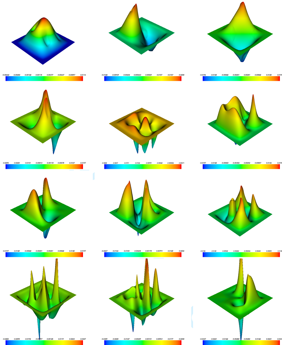
Figure 10. The 12 POD basis functions generated in the 2D numerical example. The POD functions 1-12 are ordered from top to bottom, left to right.
