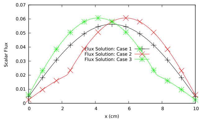
Figure 2. The 3 normalised scalar flux solutions used to generate the snapshots for the POD construction.
