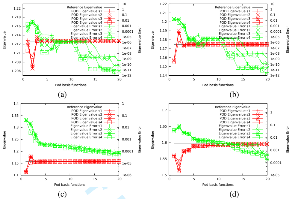
Figure 5. The graphs show the eigenvalues together with their errors when problems R1-R4 were solved using the reduced order models with varying POD basis sizes. Graphs (a-d) correspond to the results for solving problems R1-R4, respectively.
